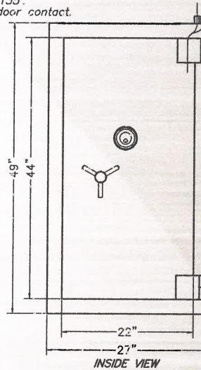
INSIDE VIEW
